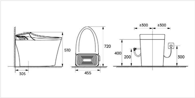
DIMENSION DRAWING
