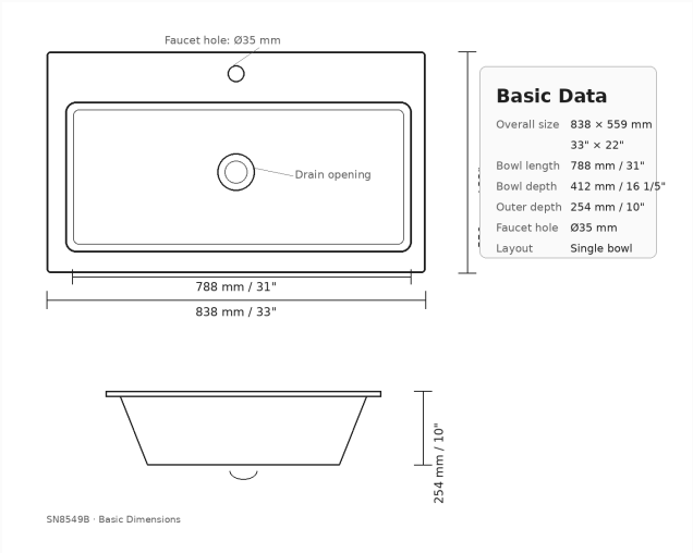
DIMENSION DRAWING · INCH [MM]
