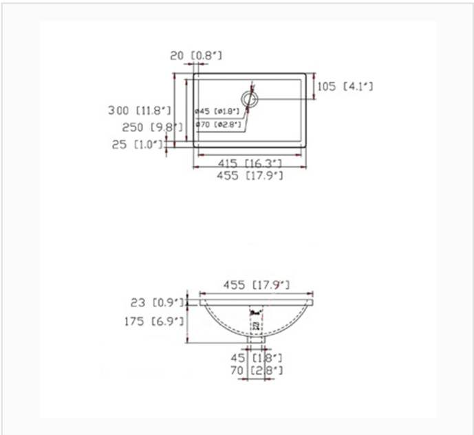
DIMENSION DRAWING · INCH [MM]
