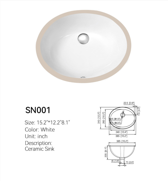
DIMENSION DRAWING · INCH [MM]
