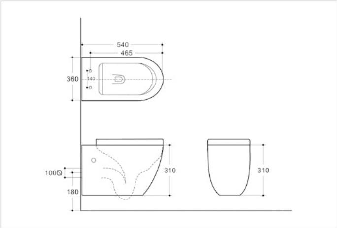
DIMENSION DRAWING · MM
