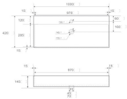
SN165 Size: 1000x425x145mm Color: White Unit: MM Description: Ceramic Sink
