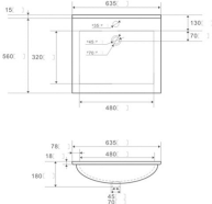
SN1558A Size: 640x560x190mm Color: White Unit: MM Description: Ceramic Sink
