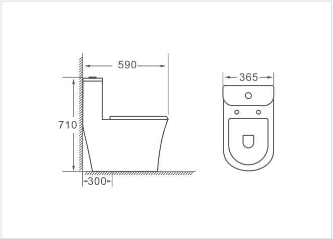
DIMENSION DRAWING
