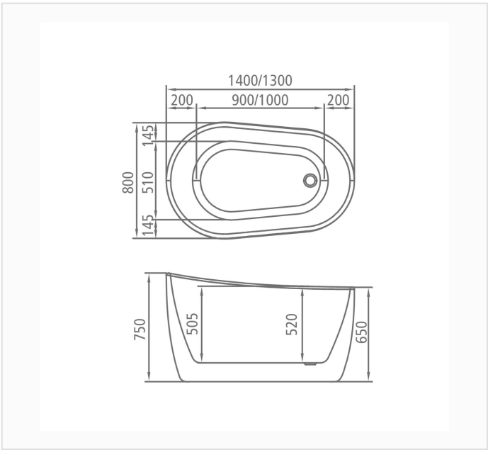
DIMENSION DRAWING · MM
