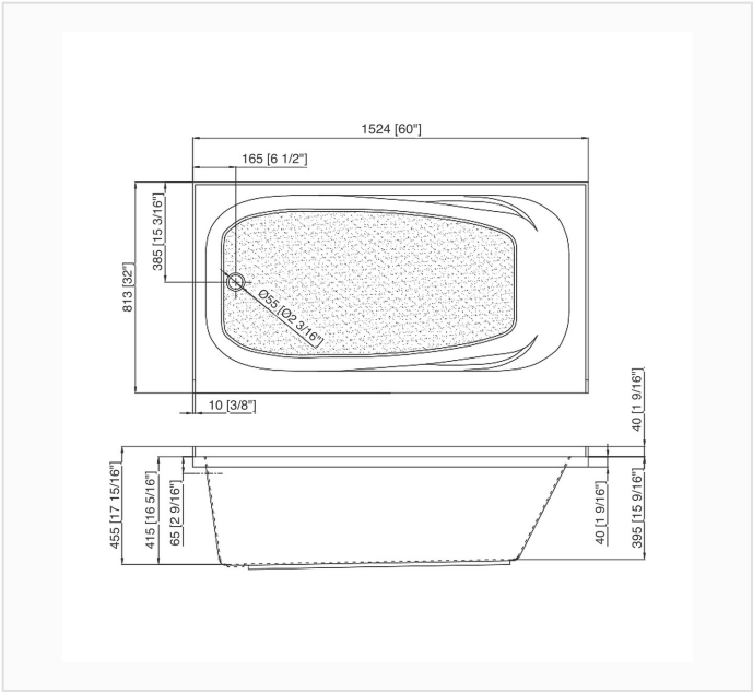
DIMENSION DRAWING · MM [IN]
