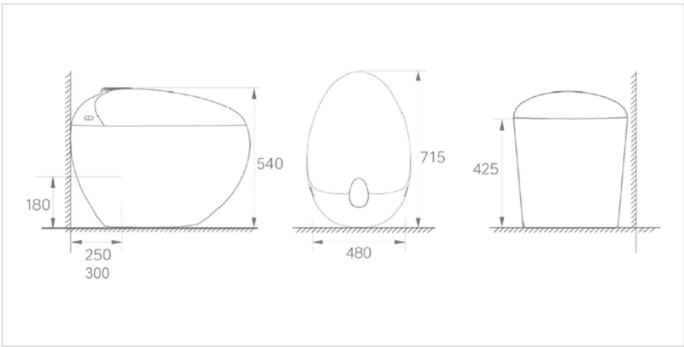
DIMENSION DRAWING
