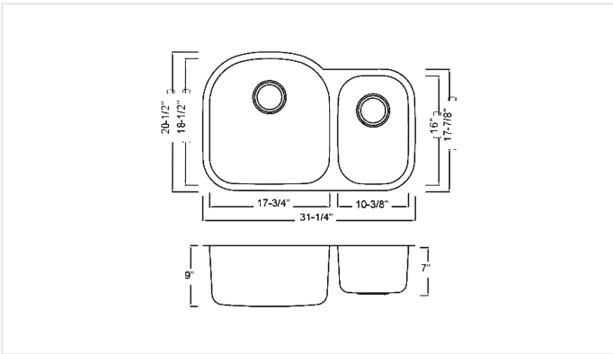
DIMENSION DRAWING
