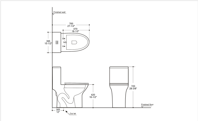
DIMENSION DRAWING
