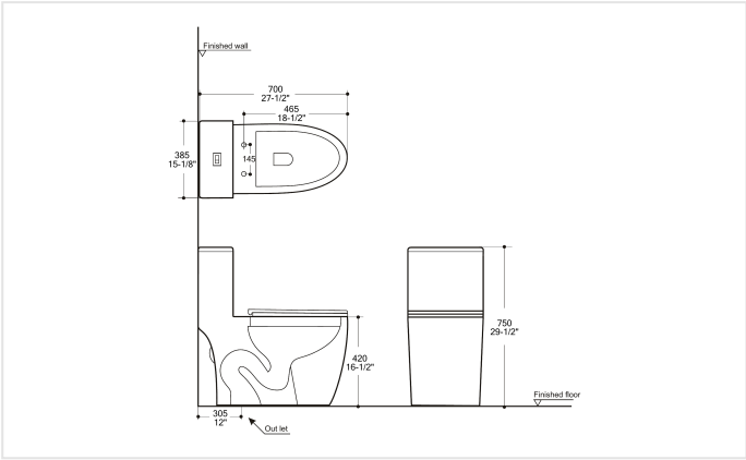
DIMENSION DRAWING
