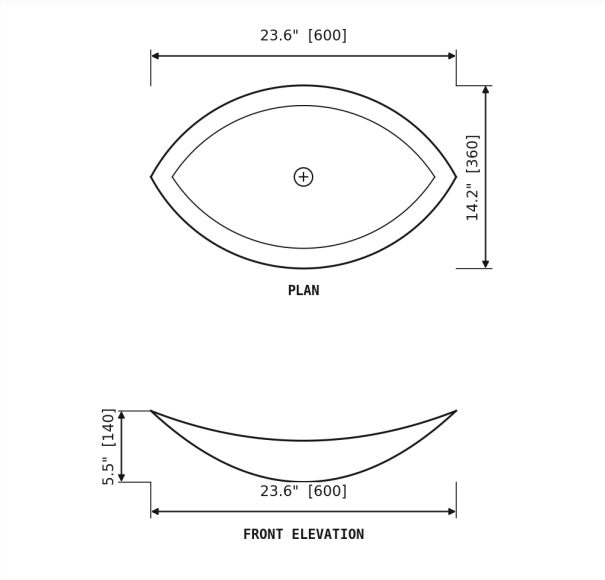
DIMENSION DRAWING · INCH [MM]
