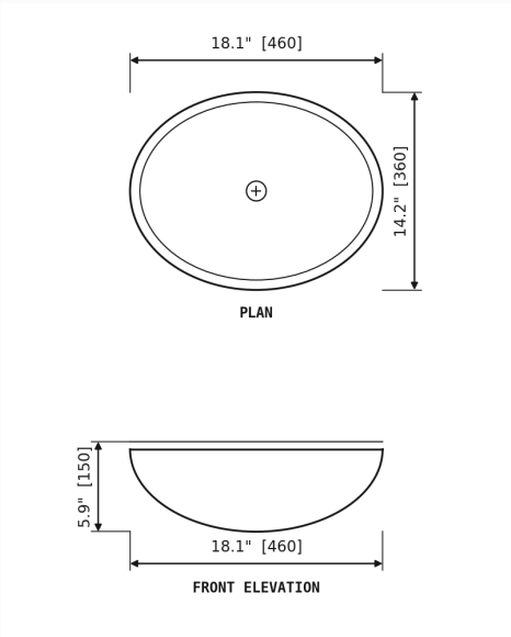
DIMENSION DRAWING · INCH [MM]
