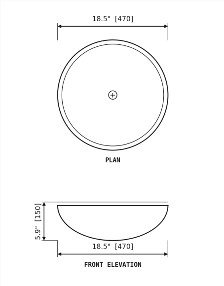
DIMENSION DRAWING · INCH [MM]
