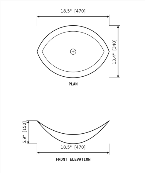
DIMENSION DRAWING · INCH [MM]
