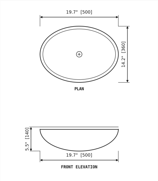
DIMENSION DRAWING · INCH [MM]
