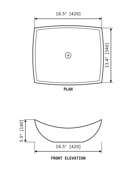
DIMENSION DRAWING · INCH [MM]
