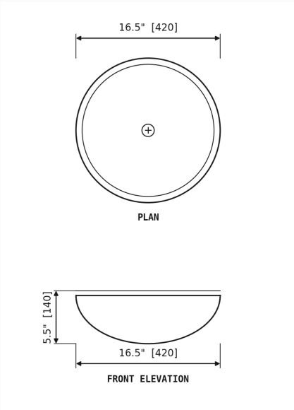
DIMENSION DRAWING · INCH [MM]
