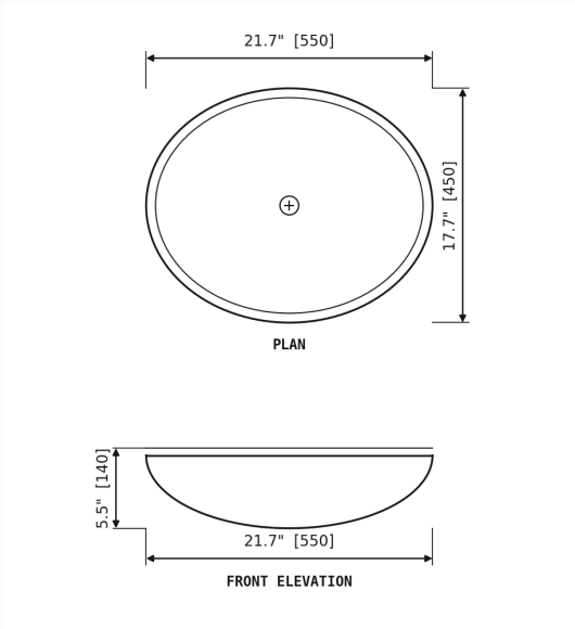
DIMENSION DRAWING · INCH [MM]
