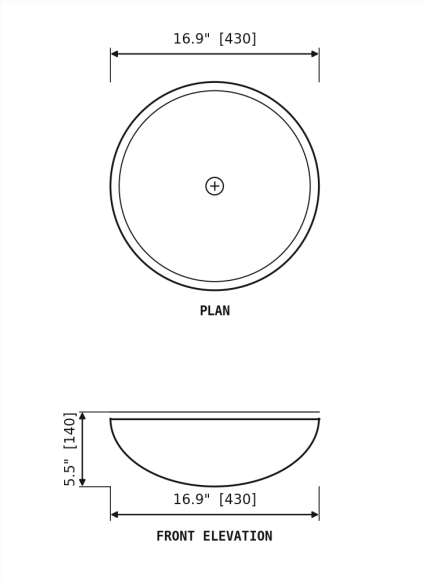
DIMENSION DRAWING · INCH [MM]
