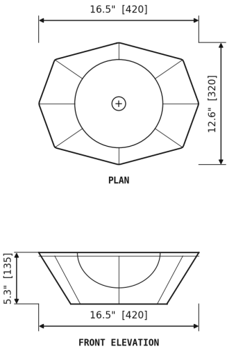
DIMENSION DRAWING · INCH [MM]
