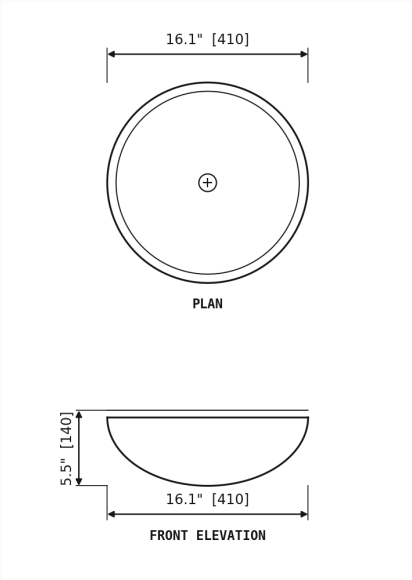
DIMENSION DRAWING · INCH [MM]
