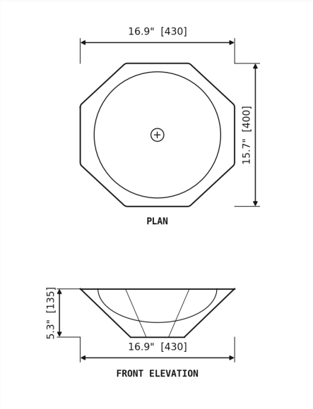
DIMENSION DRAWING · INCH [MM]
